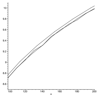
Figure 4: A plot of the formula for unbiased binary tries compared to simulation results for the unbiased binary source and for 24 bit integers.
