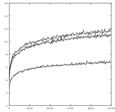
Figure 7: Plot of the formula for the average stack-size with different choices for the excluded symbol compared to the simulation results (averaged on 20 entries).
