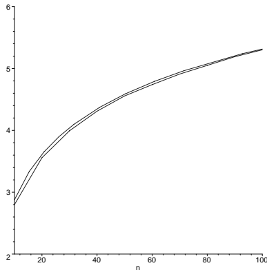
Figure 3: A plot of the formula (lowest curve of Figure 2) compared to simulation results.
