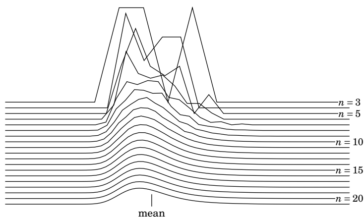
Figure 8: This figure shows the distributions of the normalized number of comparisons for small n . The distributions are computed by unfolding the distributional recurrence (4.12). This figure serves as visual evidence for the convergence of cost distributions to a limit law. It is heavily inspired by a corresponding figure for classic Quicksort [Sedgewick and Flajolet, 1996, Figure 1.3].
