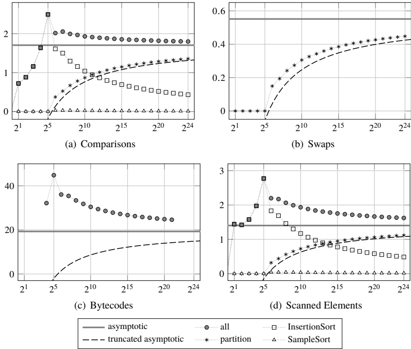
Figure 6 Comparison, swap, Bytecode and scanned element counts ( \dots\bullet\dots ) normalized by n \ln n , for \text{YQS}_t^w with \mathbf{t} = (1, 1, 1) and w = 46 against the leading-term asymptotic \frac{a}{H} n \ln(n) (—) from Theorem 4.1 and its truncated version \frac{a}{H} n \ln(\frac{n}{w}) (- - -). For comparisons and scanned elements, the contributions from PARTITION ( \dots*\dots ), INSERTIONSORT ( \dots\square\dots ) and SAMPLESORT ( \dots\triangle\dots ) are also given separately. Note that swaps only occur during partitioning (Insertionsort uses single write accesses). For reasonably large n , the main contribution indeed comes from PARTITION, however, INSERTIONSORT on short subarrays also contributes significantly. This is probably true for all cost measures, even though not shown here in detail.
