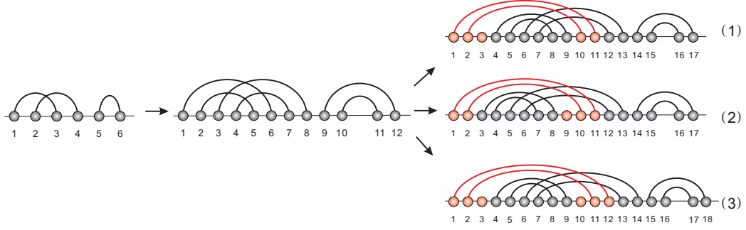
Figure 6: The first inflation step a shape (left) is inflated to a 3-noncrossing, 2-canonical structure. First, every arc in the shape is inflated to a stack of size at least two (middle), and then the shape is inflated to a new 3-noncrossing, 2-canonical structure (right) by adding one stack of size two. There are three ways to insert the isolated vertices.
