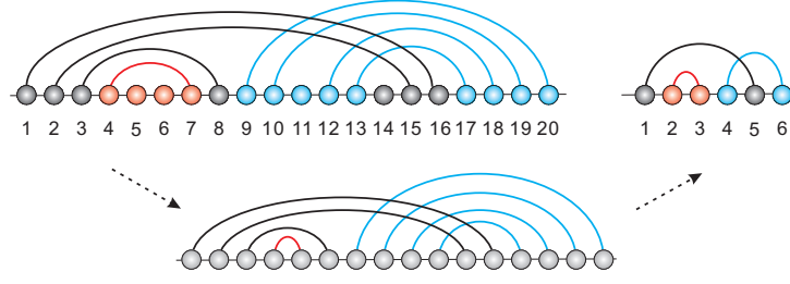
Figure 5: A 3-noncrossing, 2-canonical RNA structure (top-left) is mapped into its shape (top-right) in two steps. A stem (blue) is mapped into a single shape-arc (blue). A hairpin-loop (red) is mapped into a shape-1-arc (red).
